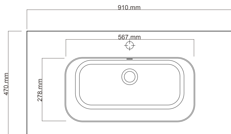
TOP WASHBASIN VIEW
