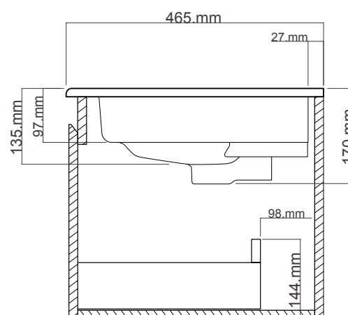
SIDE WASHBASIN VIEW
