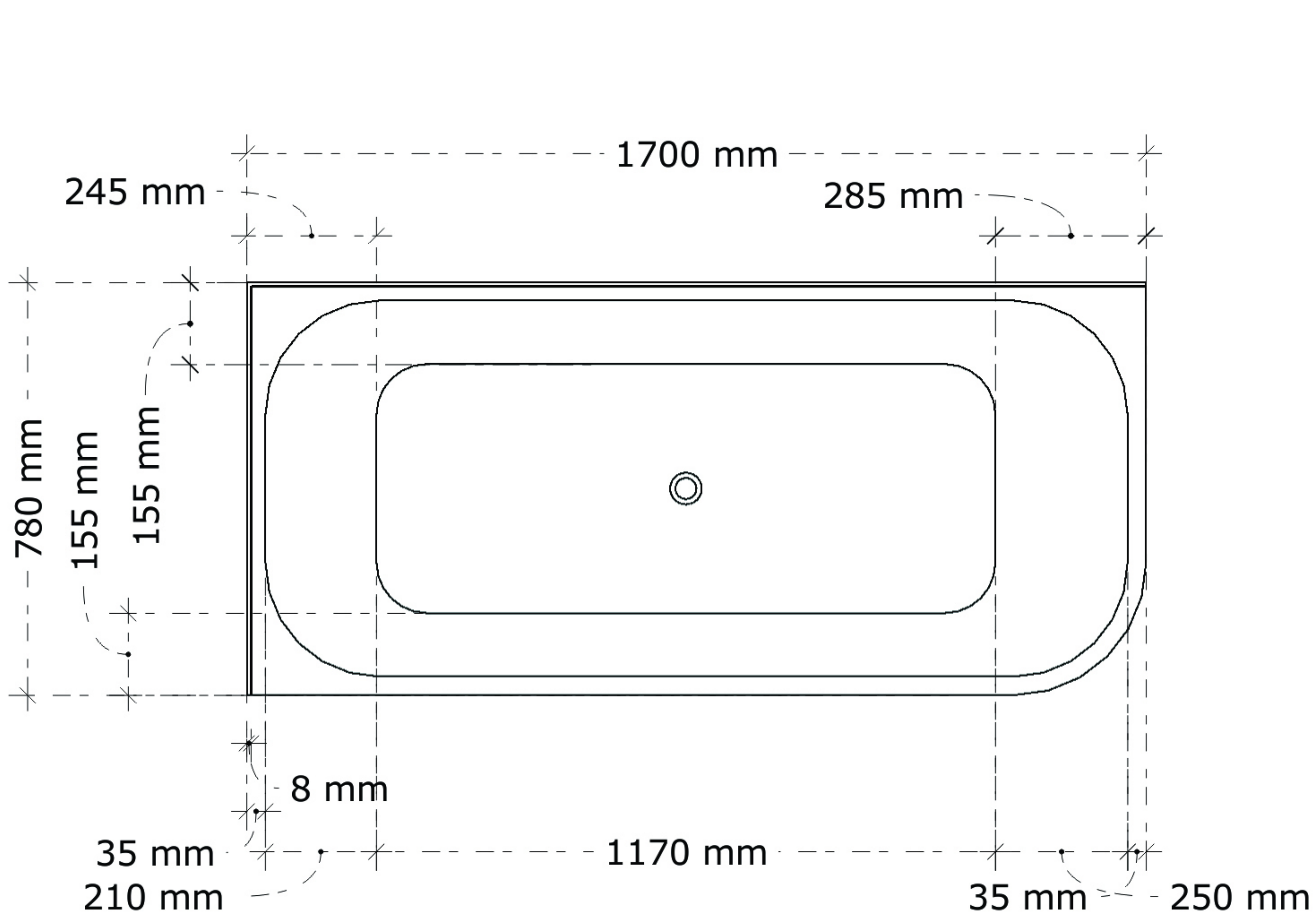
TOP VIEW
