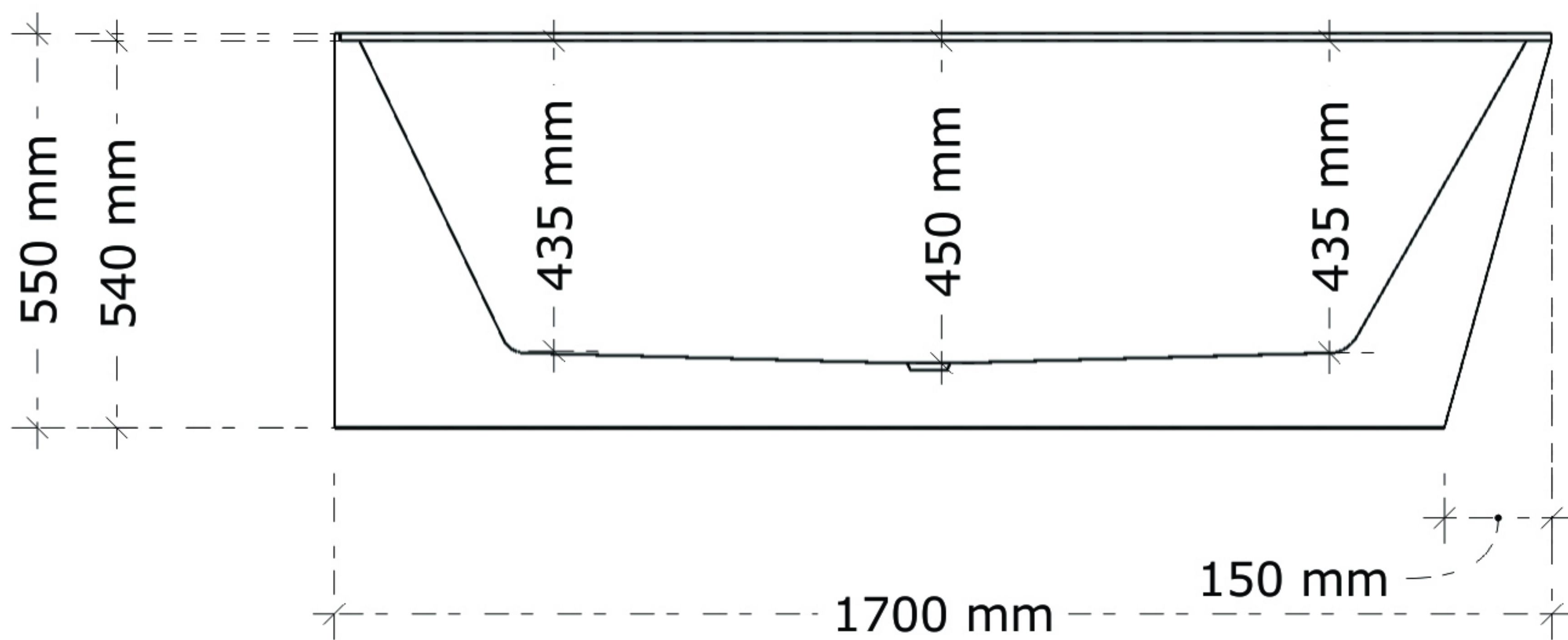
FRONT VIEW
