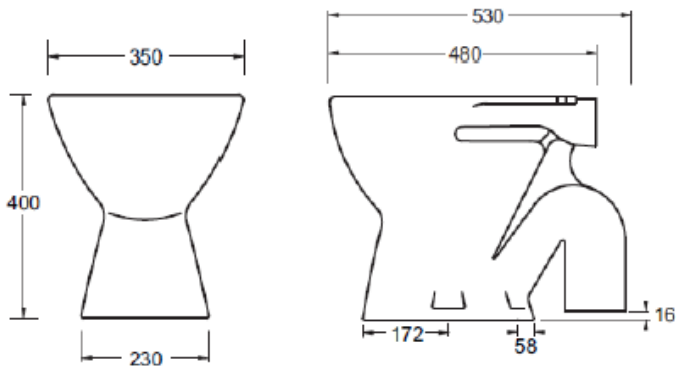
S Pan Dimensions
