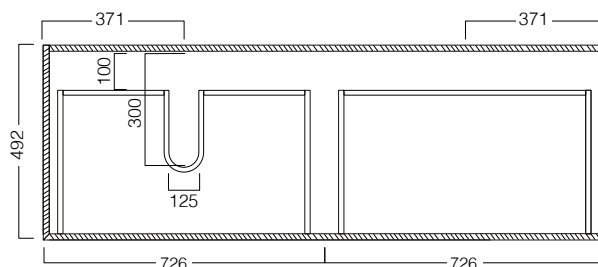
Side Section
