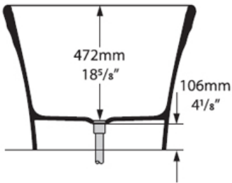
Section BB Shown with K12/K40 waste kit
