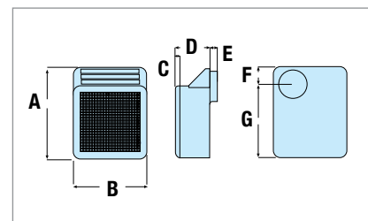
▶ Dimensions - Multi-Vent (Surface Mount)
