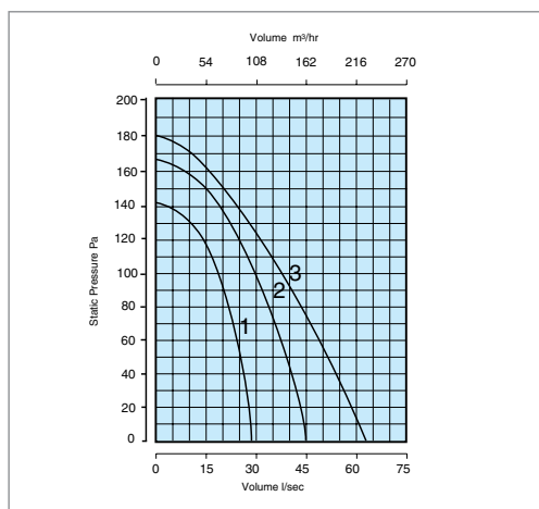
▶ Performance - Multi-Vent
