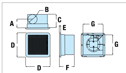
▶ Dimensions - Multi-Vent (Flush Fitting)
