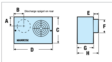
▶ Dimensions - CF200
