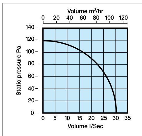
▶ Performance - CF200
