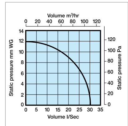
▶ Performance - SF200
