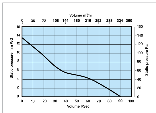
▶ Performance - SF150
