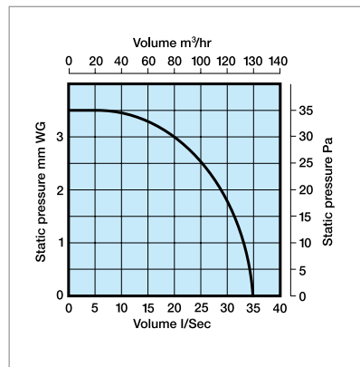
▶ Performance - SF125
