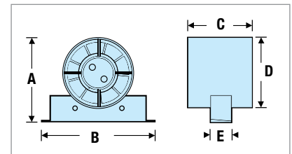
▶ Dimensions - SF200
