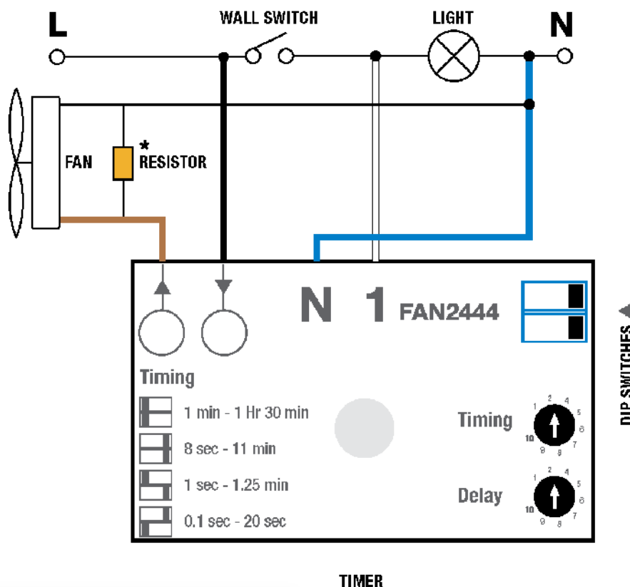
TIMER
