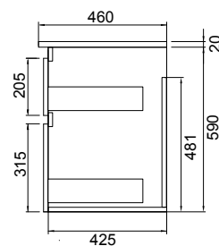
Side Section
