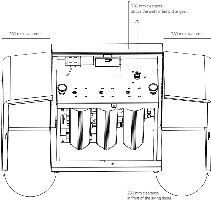
Fig 6. Installation Clearance
