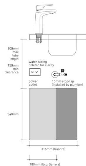
Preferred Eco, Quadra & Sahara installation layout
