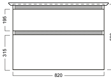
Top Section
